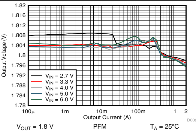
Figure 15. Output Voltage versus Output Current
