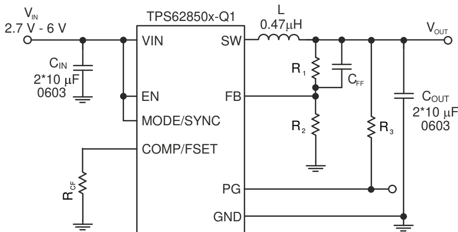
Figure 4. Typical Application
