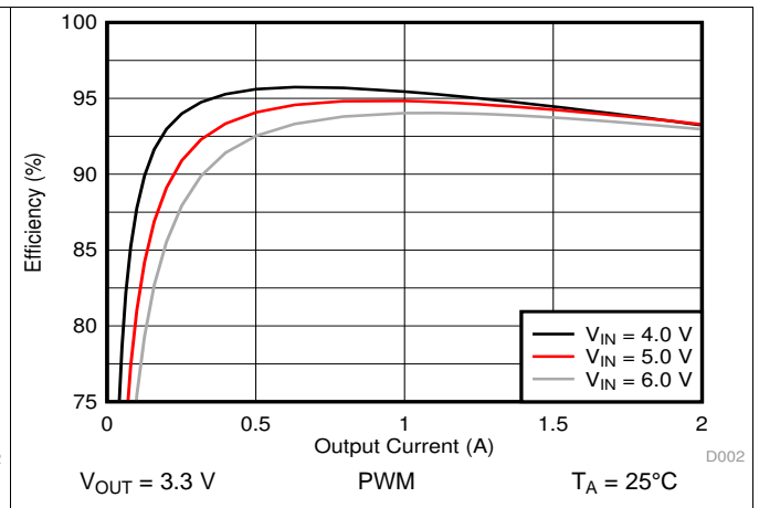
Figure 6. Efficiency versus Output Current
