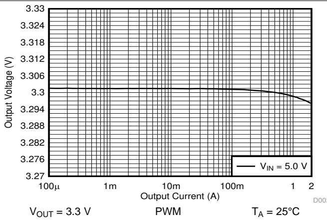
Figure 14. Output Voltage versus Output Current
