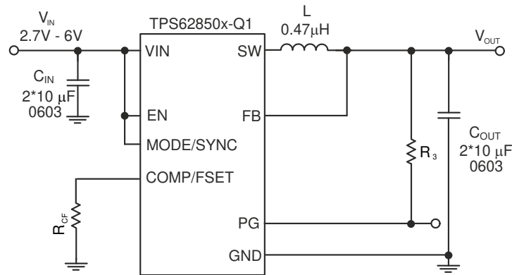
Figure 56. Schematic for Fixed Output Voltage Versions
