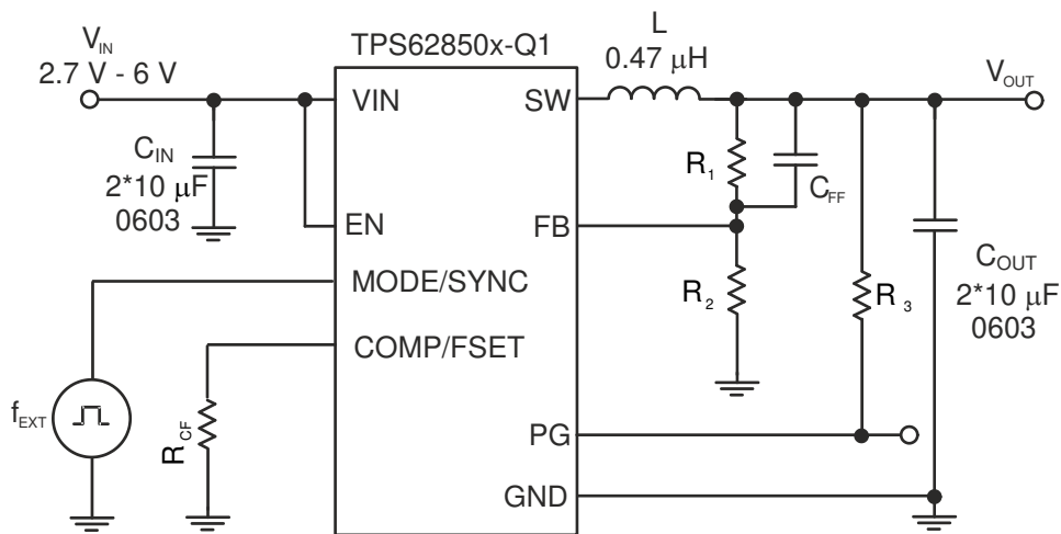
Figure 57. Schematic using External Synchronization
