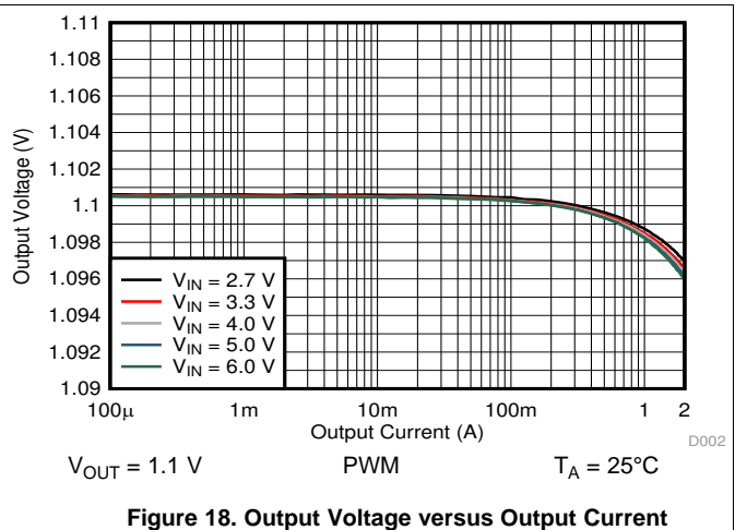
Figure 18. Output Voltage versus Output Current
