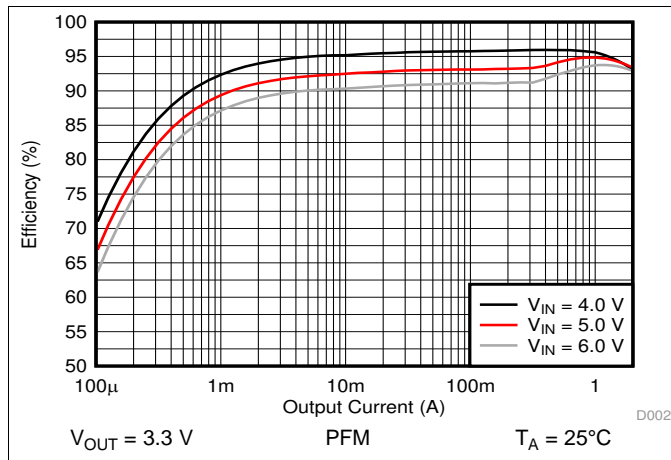
Figure 5. Efficiency versus Output Current
