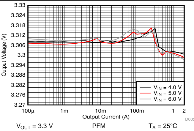
Figure 13. Output Voltage versus Output Current
