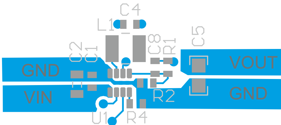
Figure 60. Example Layout
