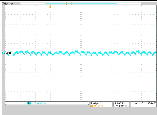
Figure 41. Output Voltage Ripple
