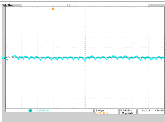
Figure 43. Output Voltage Ripple
