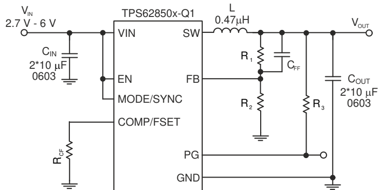
Figure 3. Measurement Setup
