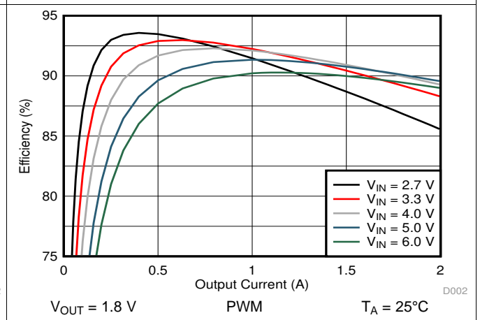
Figure 8. Efficiency versus Output Current
