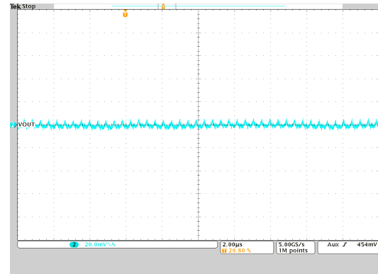
Figure 42. Output Voltage Ripple
