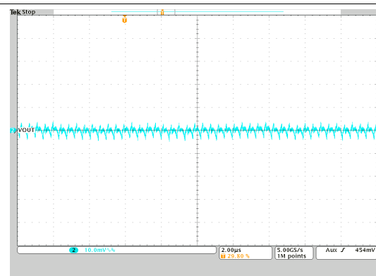
Figure 44. Output Voltage Ripple
