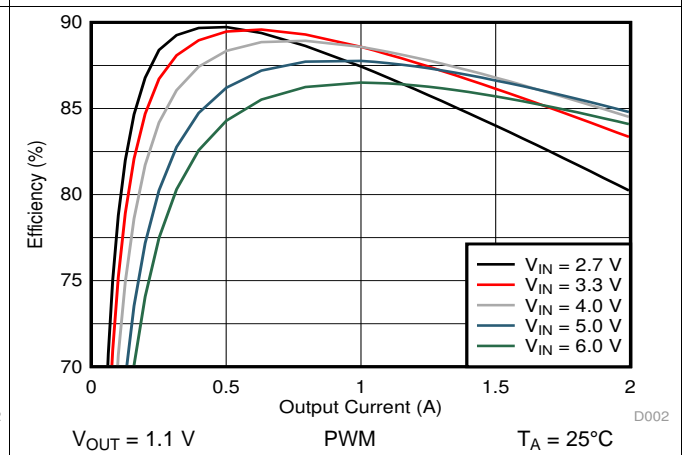
Figure 10. Efficiency versus Output Current
