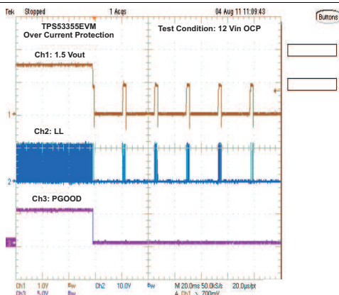
Figure 45. Output Overcurrent Protection
