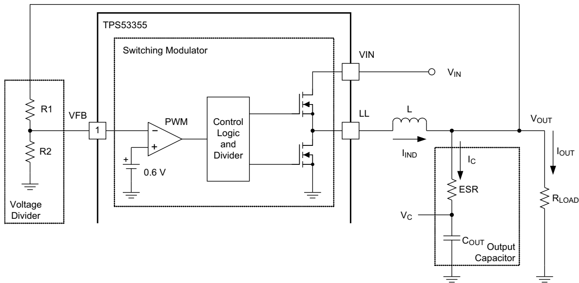
Figure 37. Simplified Modulator Model
