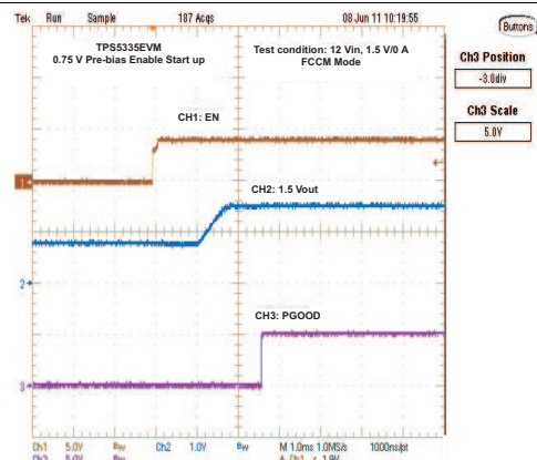
Figure 44. Output 0.75-V Prebias Turn-on
