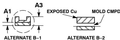
DETAIL B
