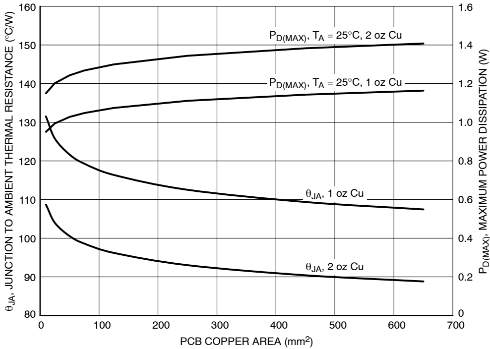
Figure 50. \theta_{JA} and P_{D(MAX)} vs. Copper Area (CSP4)
