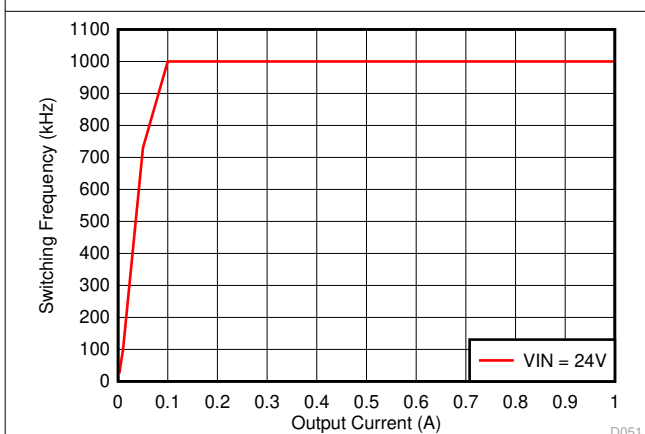
V_{OUT} = 12\text{ V} Figure 6-29. Auto PFM Mode Switching Frequency vs Output Current
