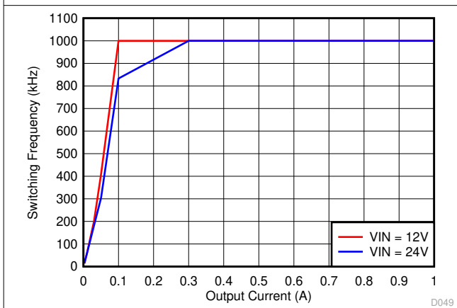
V_{OUT} = 5\text{ V} Adjustable Option Figure 6-27. Auto PFM Mode Switching Frequency vs Output Current
