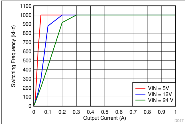
V_{OUT} = 3.3\text{ V} Adjustable Option Figure 6-25. Auto PFM Mode Switching Frequency vs Output Current
