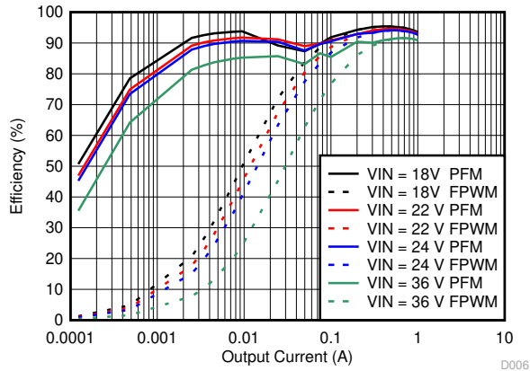
Figure 8-24. Efficiency
