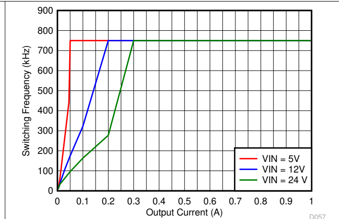
V_{OUT} = 3.3\text{ V} Fixed Option Figure 6-26. Auto PFM Mode Switching Frequency vs Output Current
