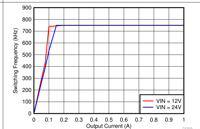
V_{OUT} = 5\text{ V} Fixed Option Figure 6-28. Auto PFM Mode Switching Frequency vs Output Current
