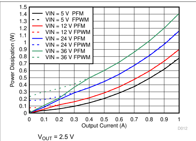
Figure 6-14. Power Dissipation
