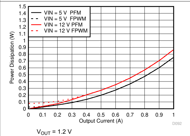
Figure 6-16. Power Dissipation
