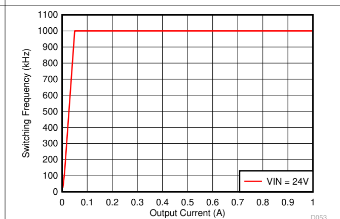
V_{OUT} = 15\text{ V} Figure 6-30. Auto PFM Mode Switching Frequency vs Output Current
