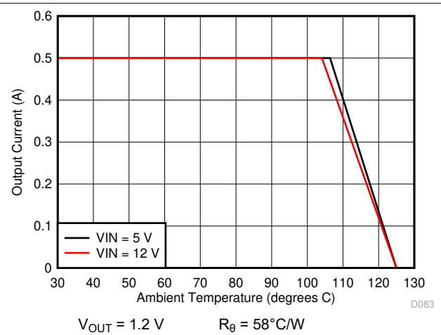
Figure 7-16. Ambient Temperature vs Output Current
