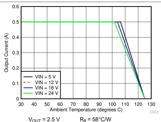
Figure 7-18. Ambient Temperature vs Output Current
