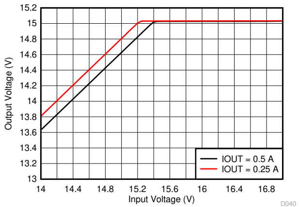
Figure 7-4. Dropout Voltage
