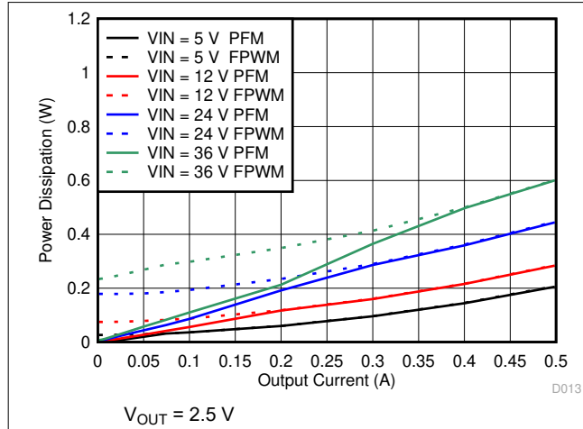
Figure 7-13. Power Dissipation
