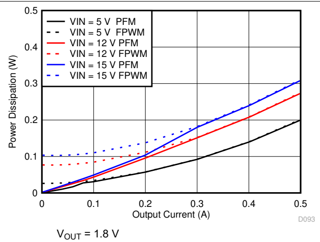
Figure 7-14. Power Dissipation
