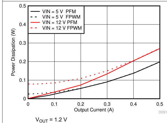
Figure 7-15. Power Dissipation
