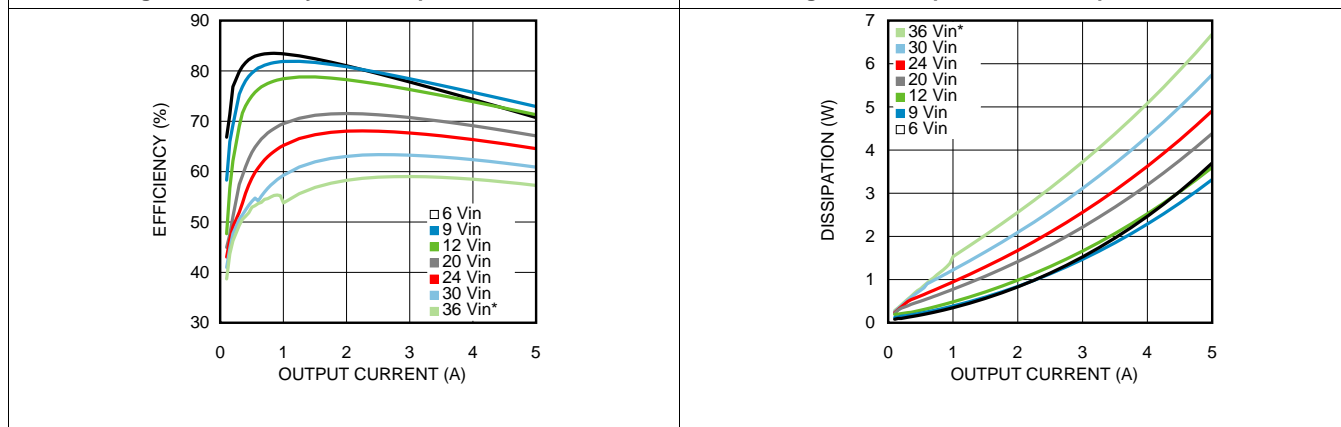
Figure 9. Efficiency 1.8-V Output at 25°C Ambient
