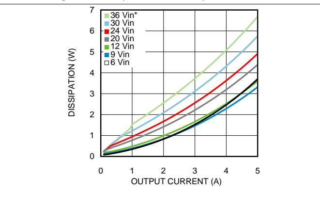
Figure 10. Dissipation 1.8-V Output at 25°C Ambient
