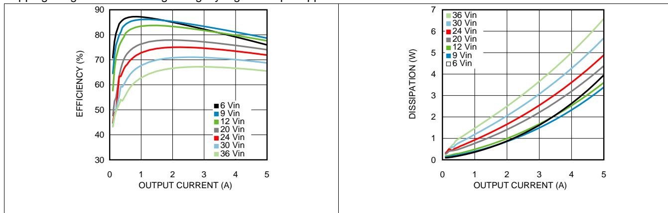
Figure 7. Efficiency 2.5-V Output at 25°C Ambient
