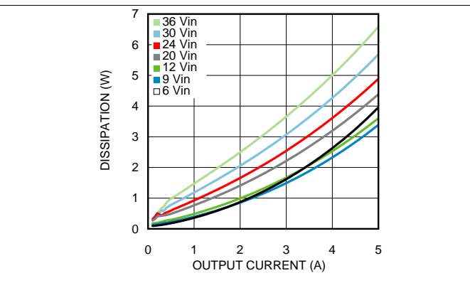
Figure 8. Dissipation 2.5-V Output at 25°C Ambient
