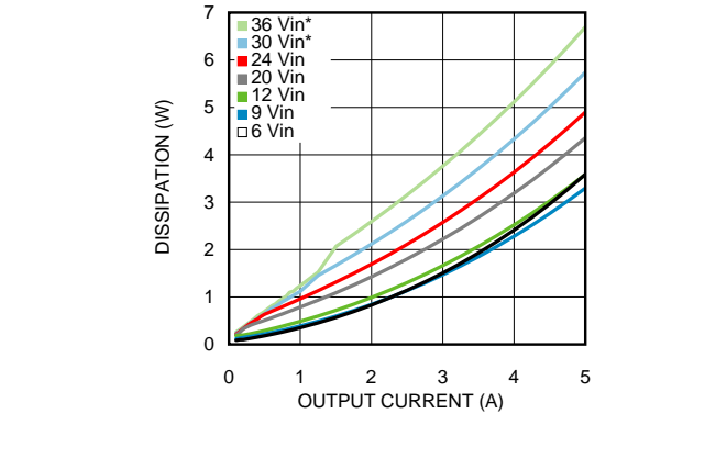
Figure 12. Dissipation 1.5-V Output at 25°C Ambient
