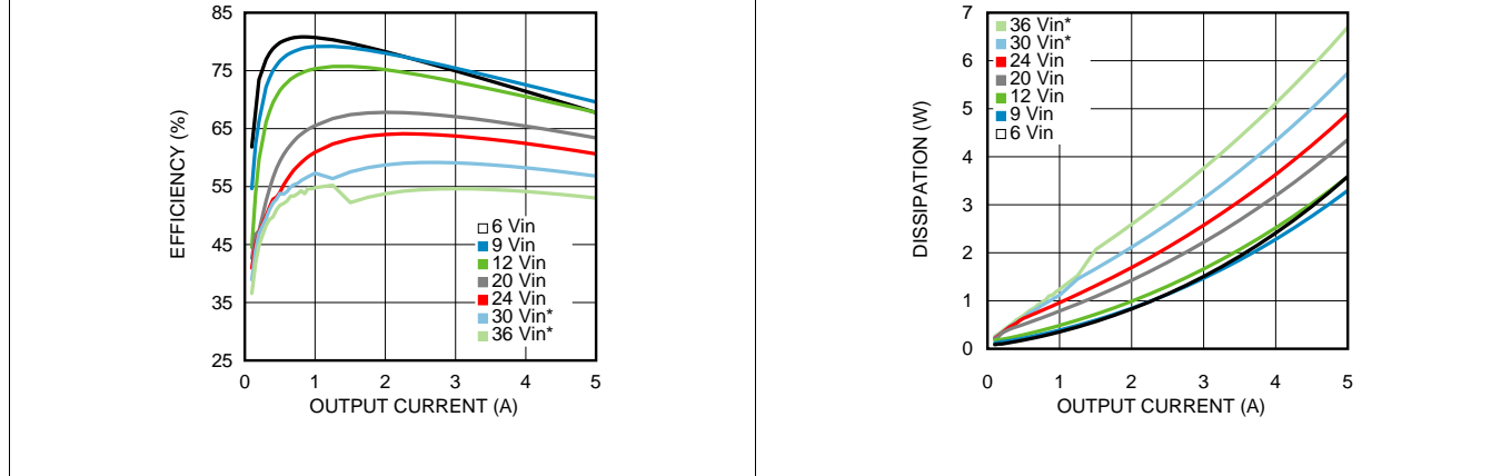
Figure 11. Efficiency 1.5-V Output at 25°C Ambient
