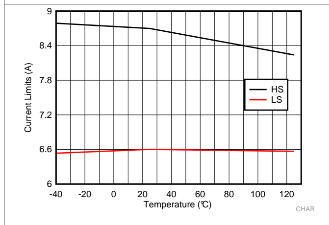
Figure 5. LM73605-Q1 High-Side and Low-Side Current Limit
