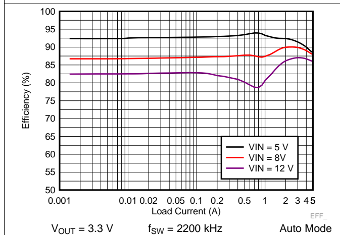
Figure 31. LM73605-Q1 Efficiency
