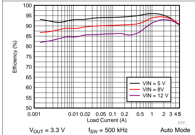
Figure 29. LM73605-Q1 Efficiency
