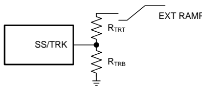
Figure 18. Soft Start Tracking External Ramp
