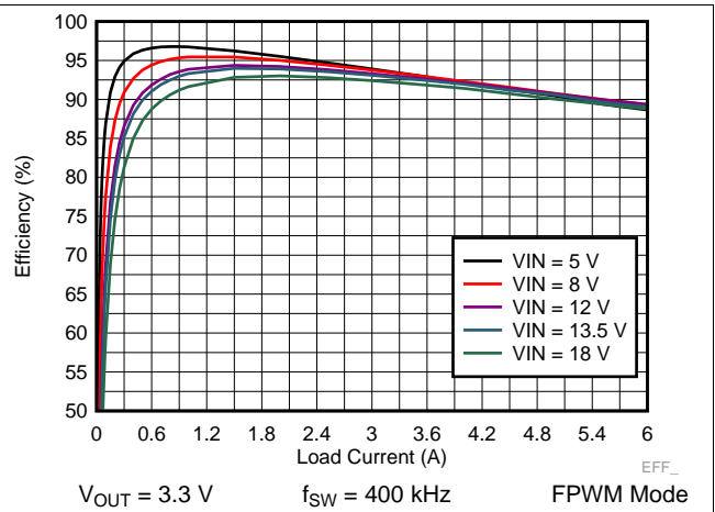
Figure 28. LM73606-Q1 Efficiency
