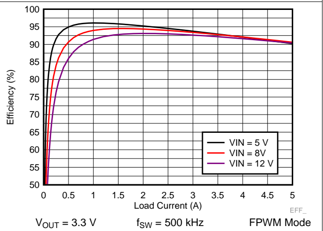
Figure 30. LM73605-Q1 Efficiency
