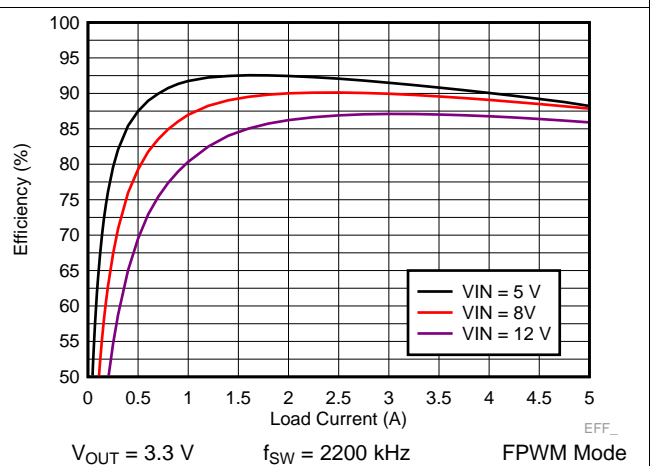
Figure 32. LM73605-Q1 Efficiency
