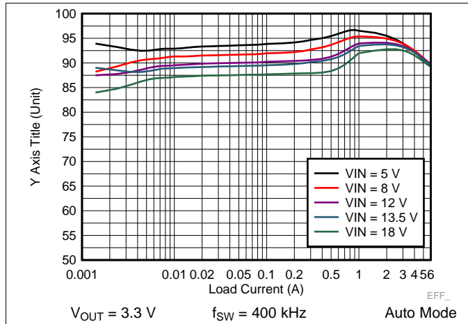
Figure 27. LM73606-Q1 Efficiency
