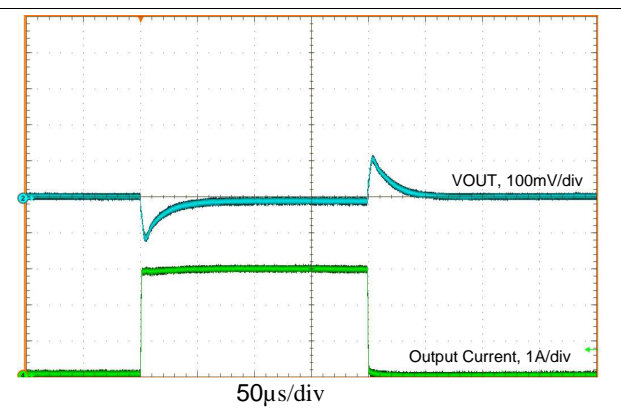
V_{OUT} = 3.3\text{ V} I_{OUT} = 0\text{ A to } 3\text{ A} , T_R = T_F = 1\ \mu\text{s} FPWM Figure 43. Load Transient
