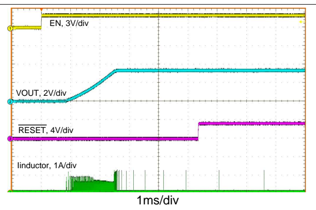
V_{OUT} = 3.3\text{ V} AUTO I_{OUT} = 0\text{ A} Figure 41. Start-Up
