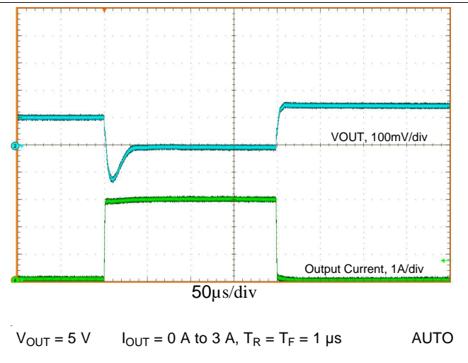
Figure 30. Load Transients
