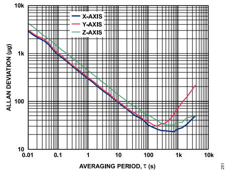
Figure 42. Root Allan Deviation
