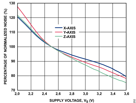
Figure 43. Normalized Noise vs. Supply Voltage, V_S
