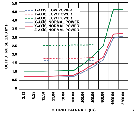
Figure 41. Noise vs. Output Data Rate for Normal and Low Power Modes, Full-Resolution (256 LSB/g)
